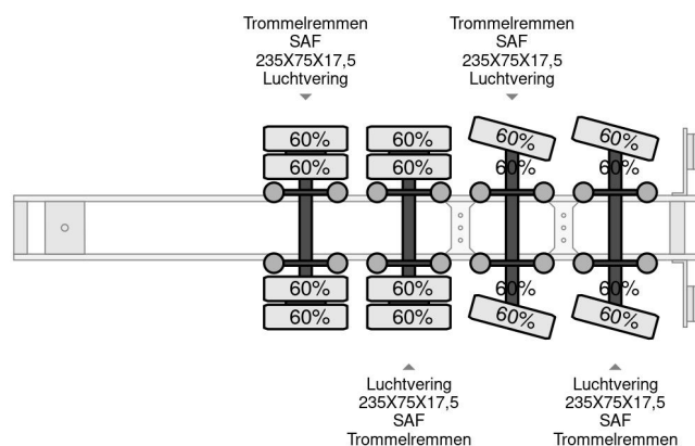
Nootboom OSDS-58-04V 4 AXLE AN 2 AXLE STEERING, 6...
