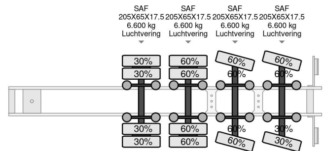
Nooteboom OSD-50-04V 2 AXLE STEERING. 6,7 METER E...
