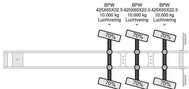
EKW 3 AXLE STEERING, DUBBLE EXTENDABLE TILL 30 ...
