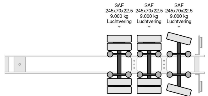
Nooteboom OSDS-48-03V LAST AXLE STEERING, 6,8 M E...
