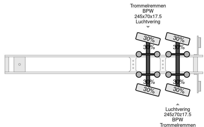
Faymonville 2 AXLE STEERING 4.3 METER EXTENDABLE
