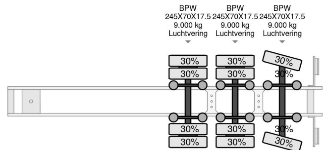
Floor 3 AXEL, 6 M EXTENDABLE, WHEEL FILLS
