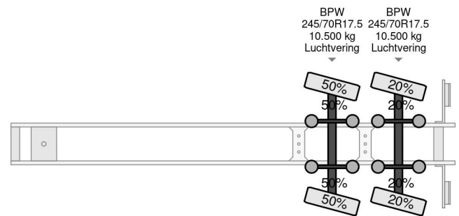
Faymonville STZ-2AA - 2 AXLES STEERING - BED: 7,40 + 3,...
