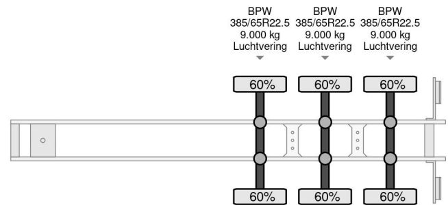
Nootboom 3 AXLE, BPW DRUM BRAKES,
