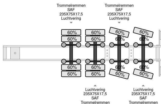
Nootboom 0SDS-58-04V 4 AXLE AN 2 AXLE STEERING, 6...
