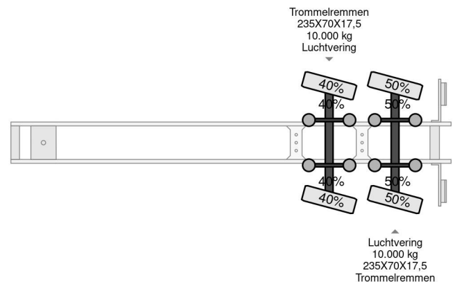
Goldhofer 2 AXEL FORCED STEERING 4,3 M EXTENDABLE...
