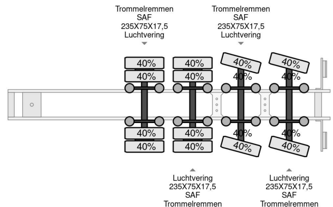
Nooteboom 0SDS-58-04V 4 AXLE AN 2 AXLE STEERING, 6...
