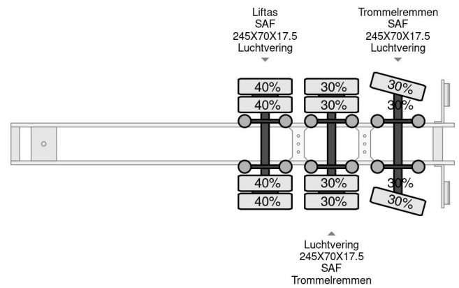
Nooteboom OSDS-48-03V, 6 M EXTENDABLE, LAST AXLE ...
