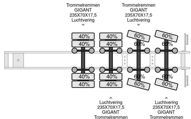
Faymonville STN--4AU LAST 2 AXLE STEERING, 6,3 M EXT...
