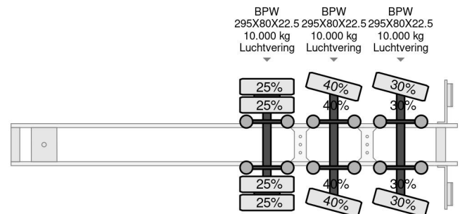
Floor HIAB ROLLER 130R
