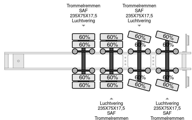
Nootboom OSDS-58-04V 4 AXLE AN 2 AXLE STEERING, 6...
