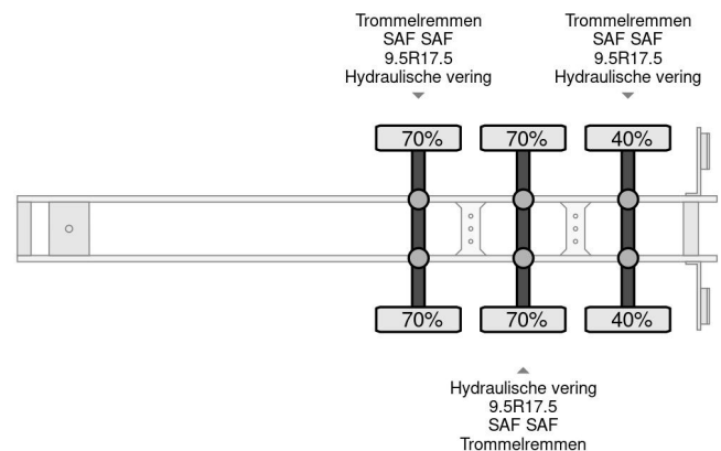
Nooteboom OSD-44-VV - 5 M EXTENDABLE + 3 AXLE SAF
