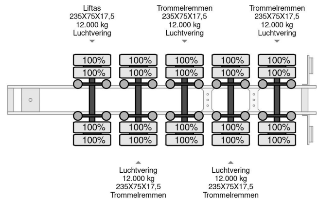
Scorpion NEW 5 AXLE 78 TON
