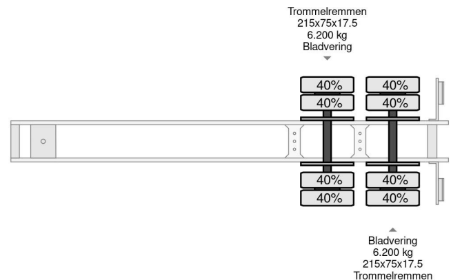
DEMICO 2 AXEL STEELSPRING
