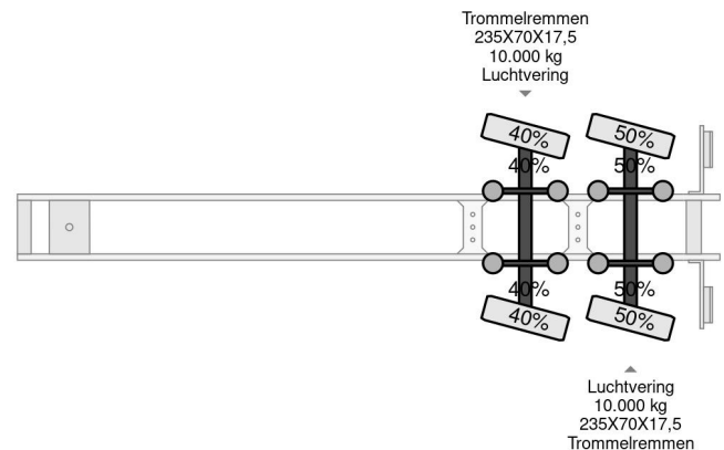
Goldhofer 2 AXLE FORCED STEERING 4,3 M EXTENDABLE
