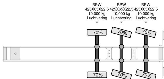
Floor HIAB ROLLER 130
