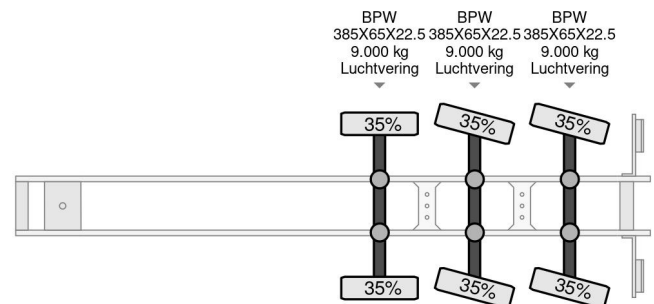
Nooteboom 3 AXEL WITH HIAB ROLLER 330 F4 HATZ ENGINE
